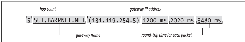
Figure 13-2. tracert output
